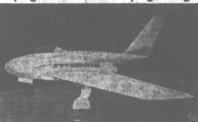
One of the smallest planes built for the USAF in recent years is the new Northrop X-4, a twin engine jet research plane now being tested at Hawthorne, Calif. Photo shows a "mock up"—a non-flying, full-scale replica of the plane. Intended to test the stability and control of tailless planes at high sub-sonic speeds, the X-4 has a wing span of only 25 feet, is 20 feet long and 15 feet high at the top of its vertical fin.
