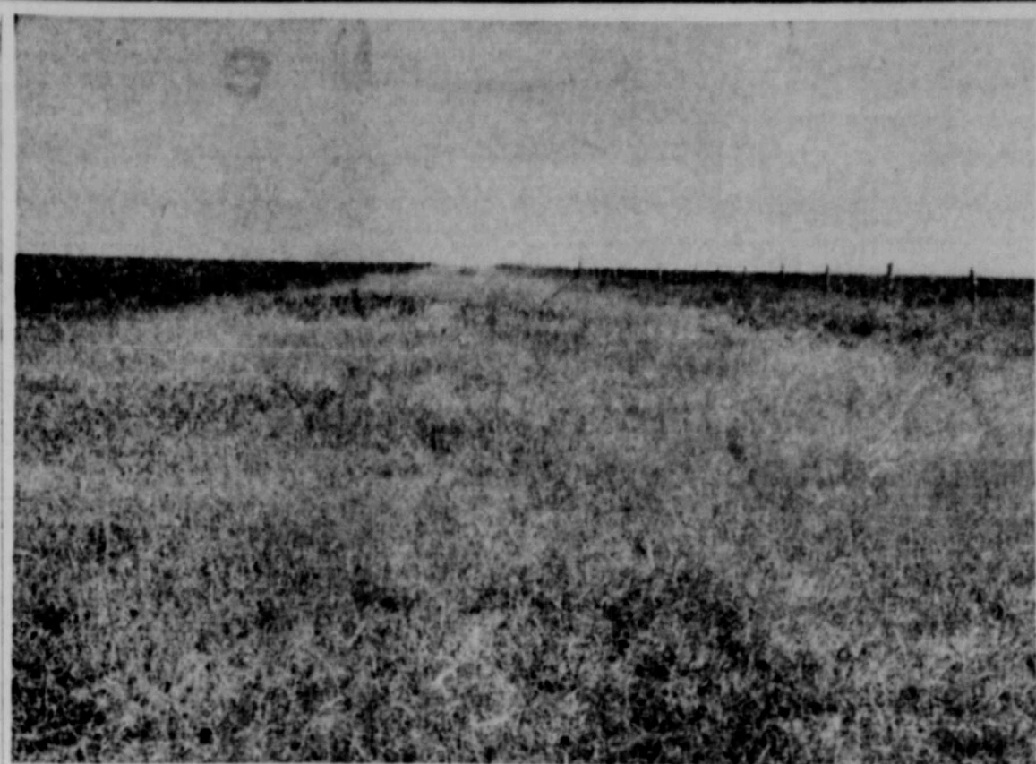
GRASSED WATERWAY—This waterway is located at the side of the field where it is least in the way of routine farming operations. There are instances where one waterway will serve several farmers. The area from which runoff water is to be handled should be carefully computed and the points at which water will enter the waterway should be planned, so that any change of size needed for the waterway can be computed so as to avoid erosion.
