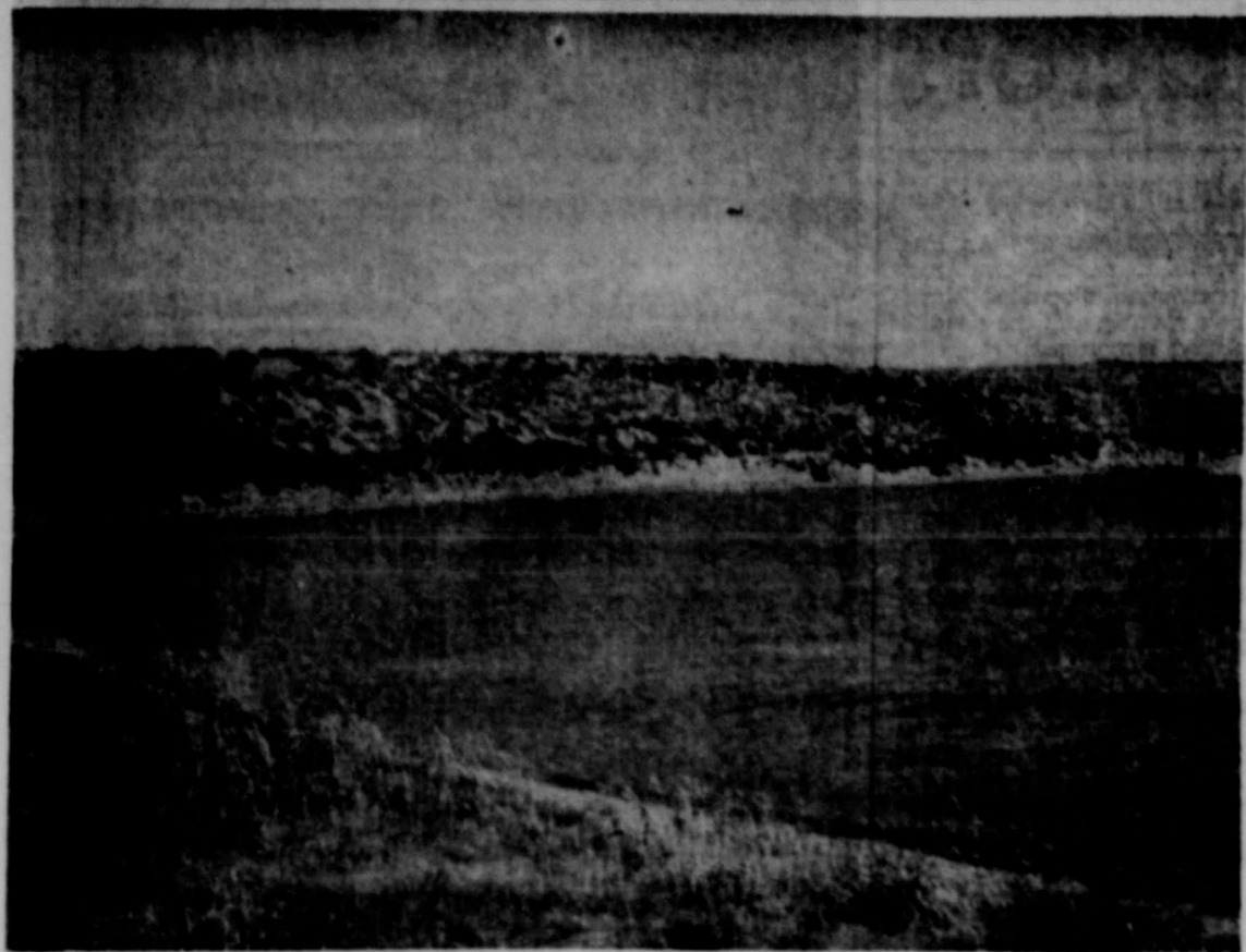
RANCH DAM —This 3,877 cubic yard dam was constructed on the Charles Dickerson ranch, about 26 miles south of Perryton, in 1951. Construction was initiated with the Ochiltree Soil Conservation District equipment. Primary purpose of this type dam is to give flood control and water for livestock.
