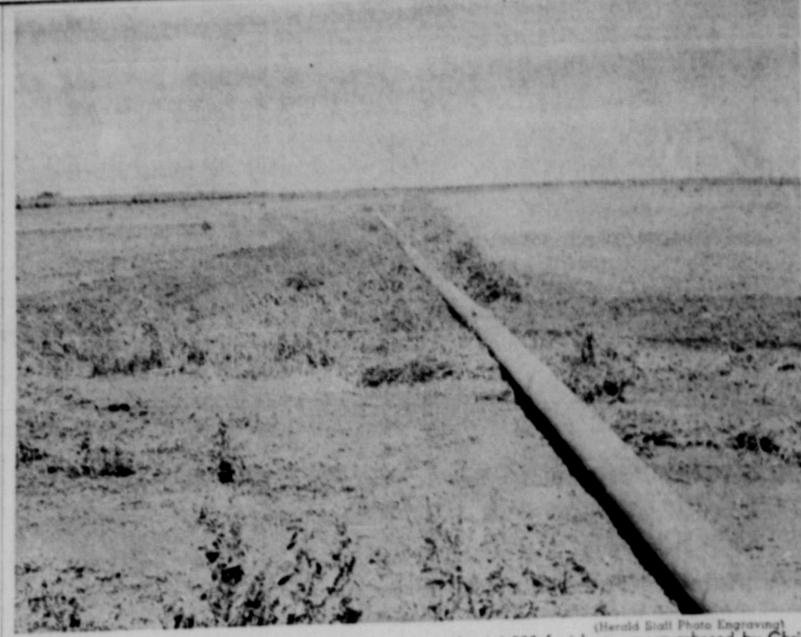
PORTABLE PIPE—This 8-inch portable aluminum pipe, about 1,000 feet long, was purchased by Chris Pshigoda and is used on the farm to convey irrigation water to 160 acres of cultivated land. The water travels about one quarter mile from the irrigation well to the field and by using the pipe, water loss through evaporation is held to a minimum, and there is no ground seepage of water between field and well.
