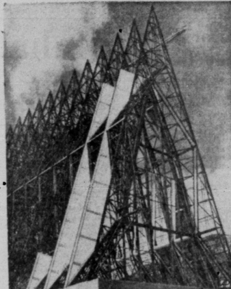
TAKING SHAPE —Aluminum panels are raised into place on the steel framework of the 17-spire chapel under construction at U.S. Air Force Academy in Colorado.
