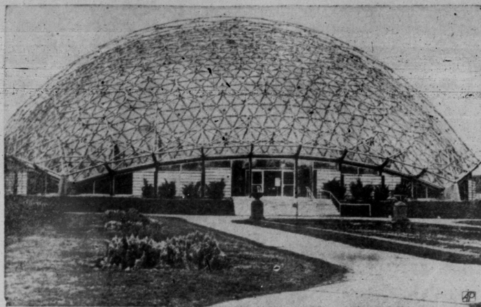
NATURE SIMULATOR —This aluminum and plexiglass structure is the 'Climatron' in the Missouri Botanical Garden in St. Louis. It is a climate control geodesic dome greenhouse, hailed as the world's most advanced botanical display house.
