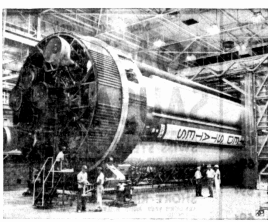
SETTING THE STAGE —Technicians work on the eight-engine SA-5 vehicle booster of the Saturn C-1 rocket at the NASA center in Huntsville, Ala. It will be part of the first Saturn with tail fins and elongated tankage for additional propellant.
