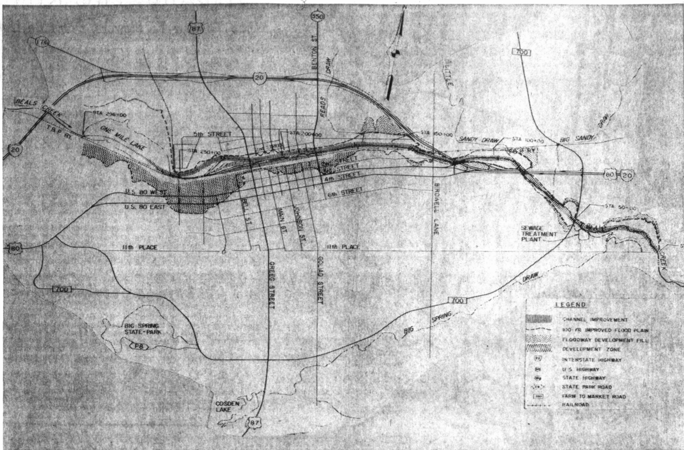
CORPS OF ENGINEERS PROPOSED FLOOD CONTROL WORK FOR BIG SPRING Various channel improvements sketched for Beals Creek, with related floodway fill and development zone
