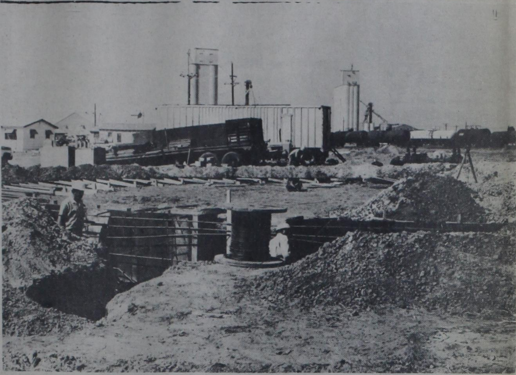
FOUNDATION WORK at the site of the city's new million gallon water reservoir was underway last week. The steel reservoir will be located just east of the county show barns. Onyx Construction Co. of Fort Worth constructed the foundation for the new tank and work on the tank itself will begin soon.
