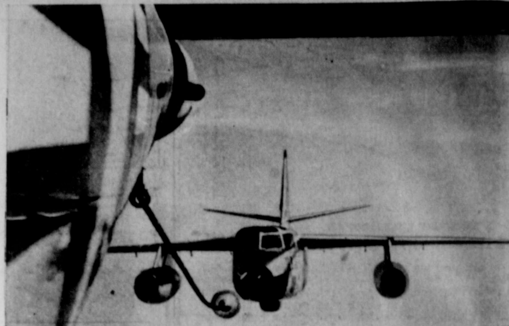
AERIAL GAS STATION —High off the South Carolina coast, an RB-66 reconnaissance bomber of the USAF Tactical Air Command moves into position for aerial refueling. The tanker aircraft is a KB-50.
