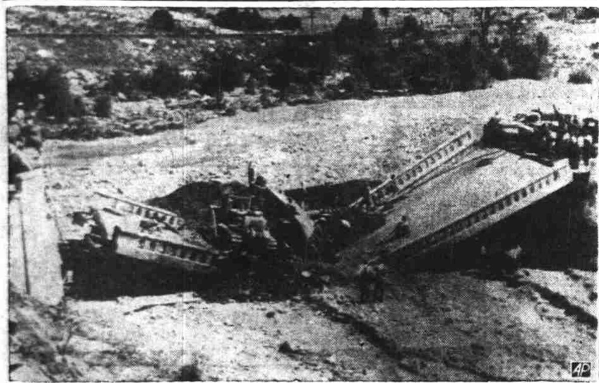
FELLED BY FLOOD — William Witherow, 25-year old Canon City, Colorado, truck driver was killed when this concrete bridge across a normally dry gulch collapsed while he was driving across it and buried him in the cab of his truck. Heavy rains had sent a flash flood surging down the gulch into the Arkansas river, undermining the center supports so that the truck's weight broke down the span, near Canon City. (AP Wirephoto).
