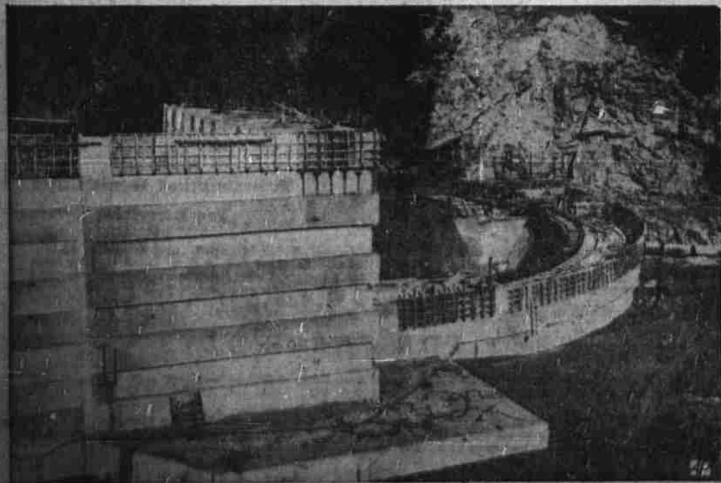
EUREKA COUNTS THE DAYS until residents will be using new water supply following completion of Eureka's $200,000 dam (above), key unit of a $2,000,000 water supply project. Arch of the dam—which is on the Eel river in Humboldt county, California—is 50 feet high but an earth fill.
