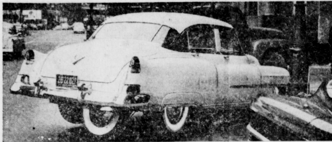
FIFTH WHEEL HELPS —Lowered by hydraulic cylinders in Detroit, the wheel acts as a jack to lift the rear wheels off the pavement in a tight-squeeze parking headache. Then a chain drive powered from the drive-shaft turns the wheel so the rear can be swung in any direction.
