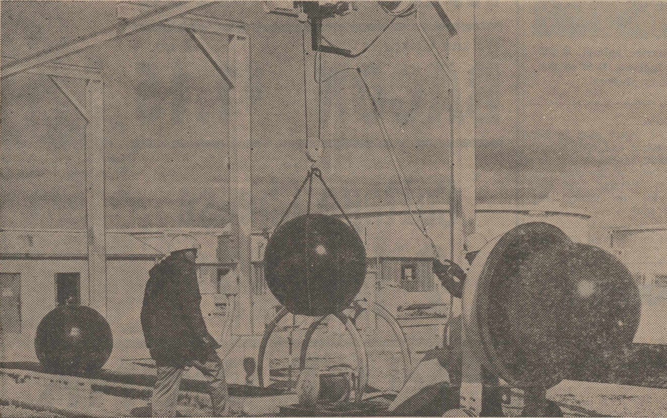
KING-SIZED RUBBER BALLS help keep crude oil pipelines running smoothly. The balls, 40 inches in diameter and weighing 900 pounds each, are sent periodically on a 630-mile trip to clean sludge and salt water from pipelines running from St. James, La., to Patoka, Ill. The new $100-million lines were completed recently.
