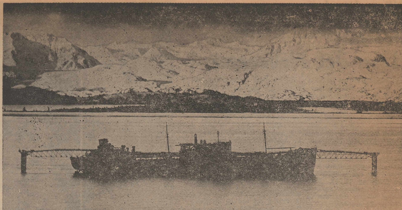
FAR-OUT FACILITY for loading crude oil sits two miles off west shore of Alaska's Cook Inlet. The unique marine terminal is capable of pumping crude oil aboard tankers at the rate of 30,000 barrels an hour.
