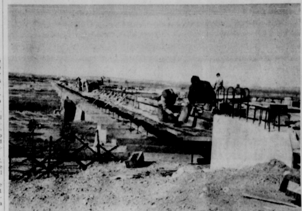
(Herald Staff Photo Engraving) NEARLY THROUGH—These workmen are shown on the last span of the new Canadian River bridge on highway 70 and the final slab is to be poured this week. Much work remains to be done on the bridge, however, and it will not be finally completed before April 15, according to latest estimates. This picture was made from the Pampa side of the river.
