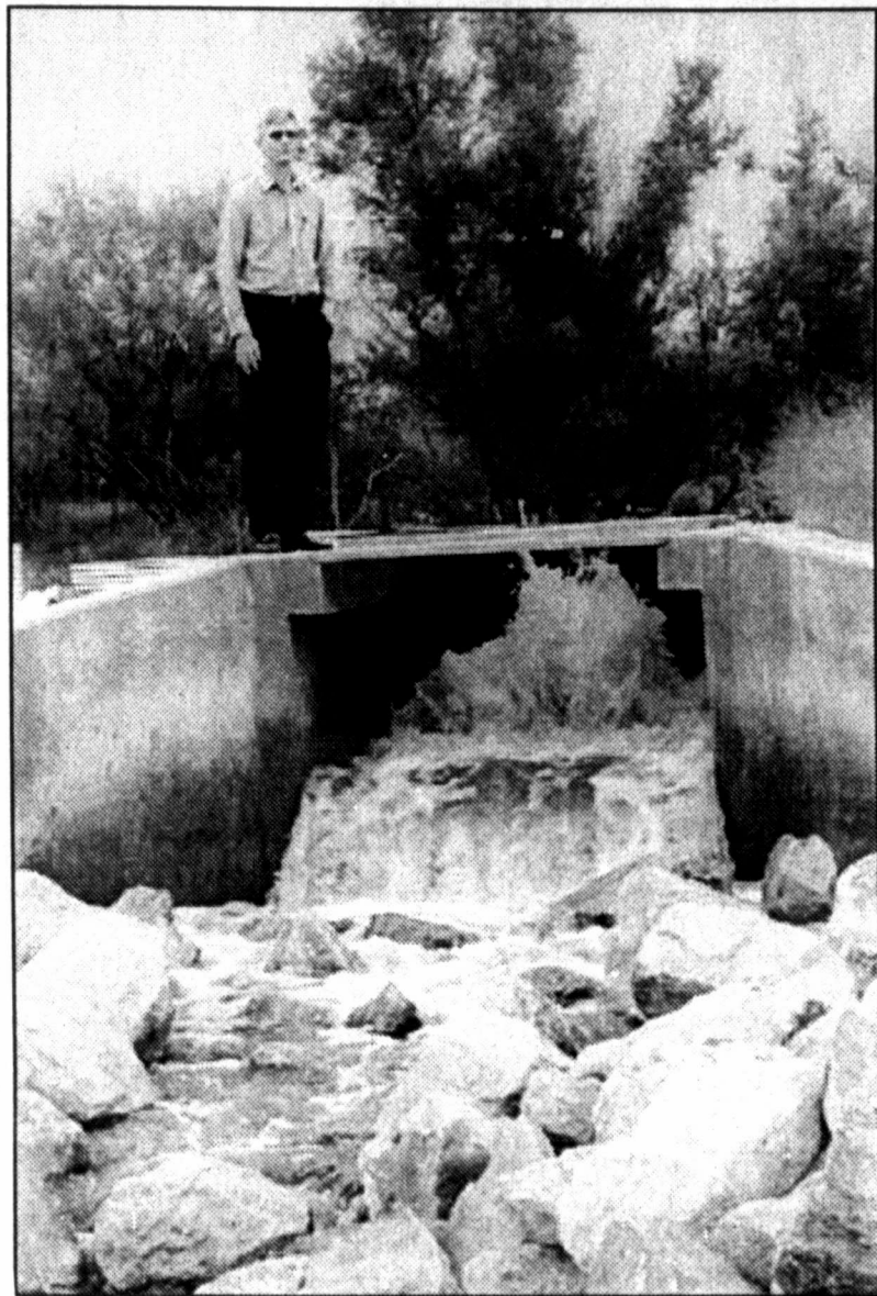
A LAKE C-CITY WATER PIPELINE is shown by Colorado River Municipal Water District official Chris Wingert, who said it flows at 5,000 gallons a minute northwest of town.
