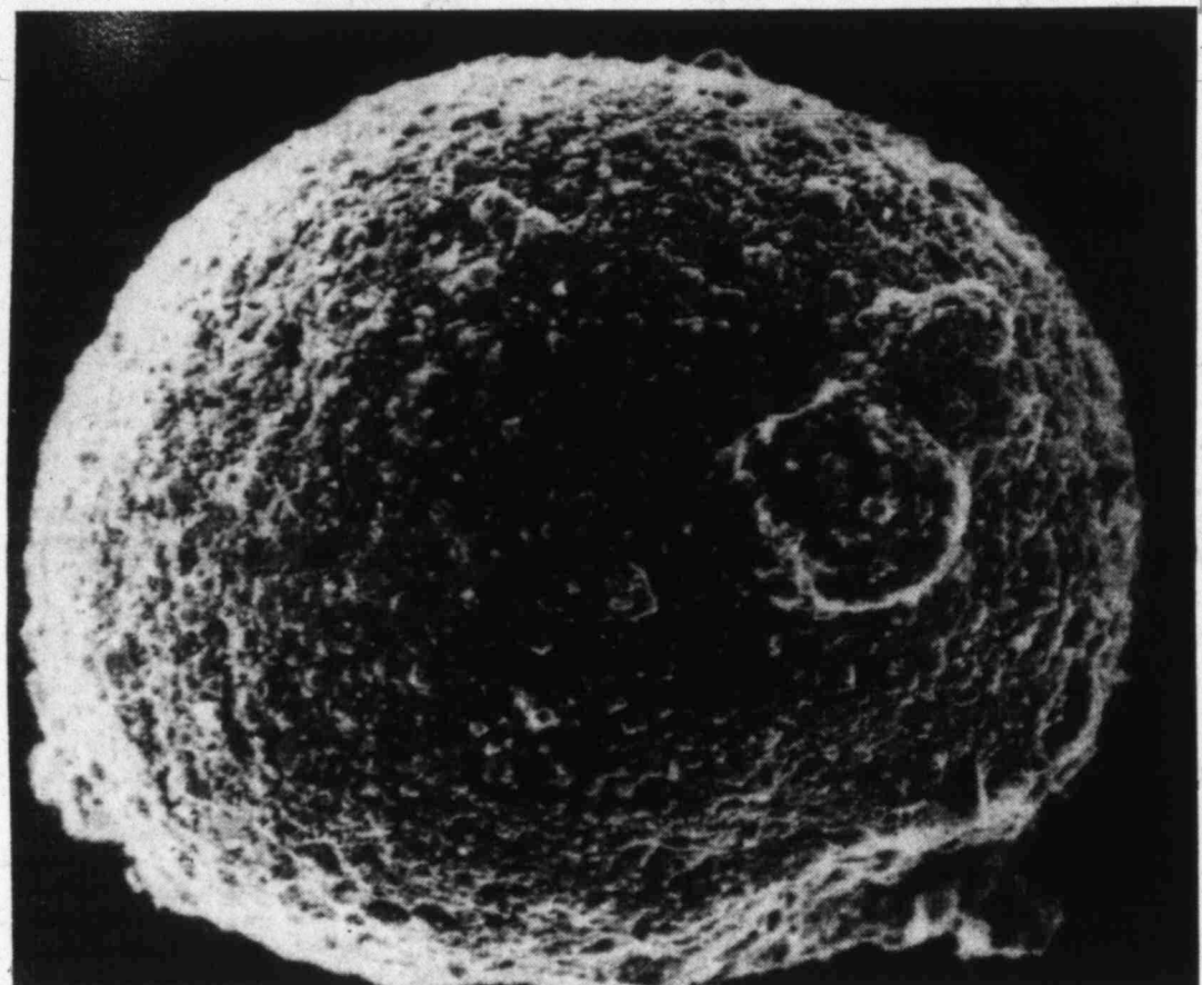
SULFUR DROPLET FROM MOUNT BAKER — This is a sulfur droplet, magnified 460 times, one of many different types of particulate material being ejected from fumaroles on Mount Baker, Washington. This droplet is less than one-one hundredth of an inch in diameter. Since about mid-March, the 10,778-foot normally quiet volcano has been geologically restless with unusually large amounts of steam and ash clouds coming from the Sherman crater on the south side of the mountain's summit. The activity has spurred a special monitoring program by scientists of the U.S. Geological Survey, the University of Washington, and the U.S. Forest Service, to try and determine the cause and nature of the activity at Mount Baker, and to define the potential hazards that could develop if an eruption should occur.
