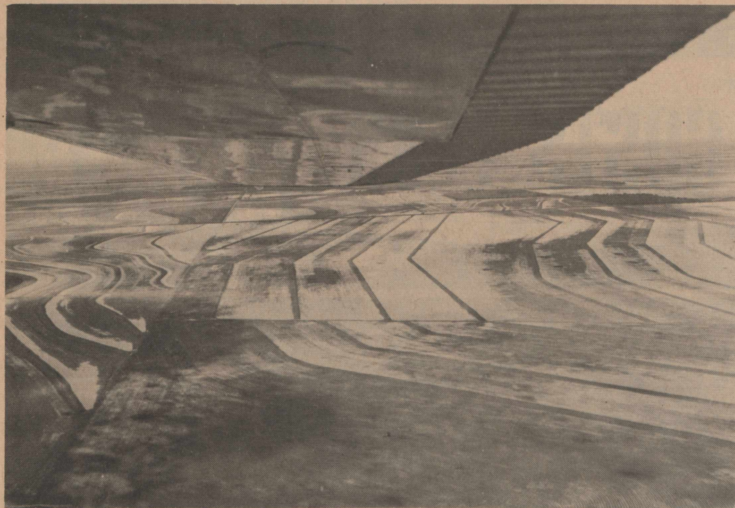
PARALLEL TERRACES--Above is an aerial view of parallel terraces on the A. C. Humphrey farm. (Photo by Soil Conservation Service.)
