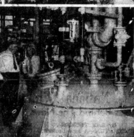
Tire & Rubber Company of Akron, Ohio, the plants have open-type walls to take advantage of Texas' benign climate and to conserve building materials. At the top left is a process building in a 60,000-ton plant while the picture beside it shows three reactors in place and space for another. Below, left, are the stripping towers which remove excess butadiene and styrene from the latex while beside it is a picture of Glenn A. Barber (white shirt), project manager for one of the plants, examining a reactor with an employee.
