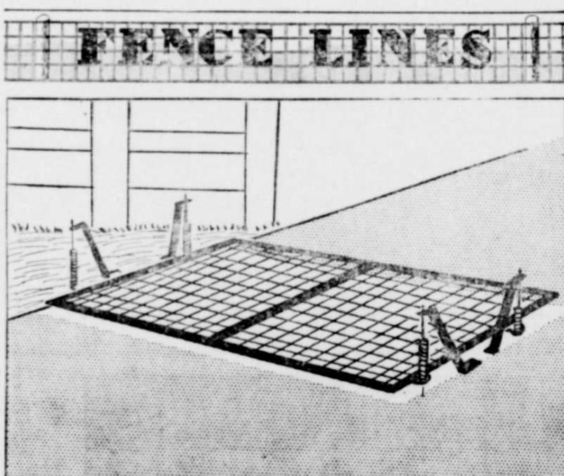
NO-CLOG GUARD ... This cattle guard will turn back any farm animal. Springs hold steel grate two inches above planks set on edge.
