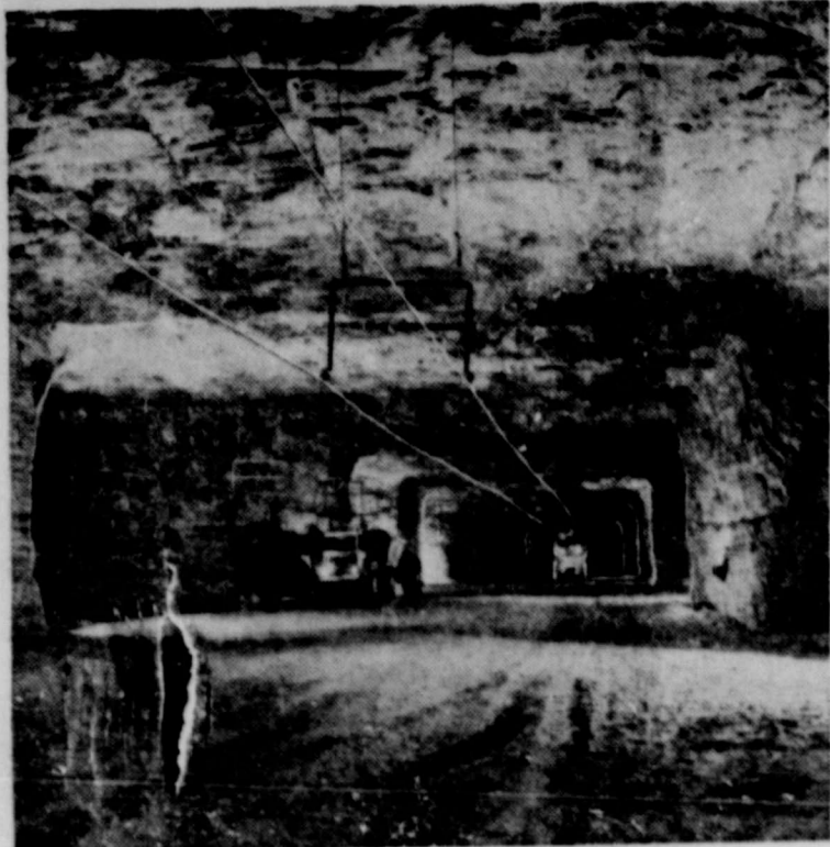
SALT MINE under metropolitan Detroit, Michigan, offers a unique civil defense opportunity for a large target city to provide both blast and fallout shelter for a substantial number of its citizens with a minimum amount of additional excavation. The mine—second largest rock salt mine in the world—is 1,137 feet under the surface. It would need more equipment and access ramps or elevators to serve as a mass shelter from attack. (Photo courtesy International Salt Co.)
