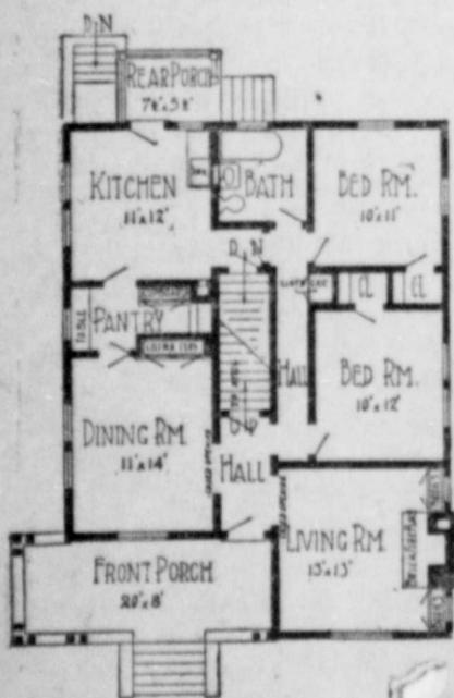
Floor Plan of Bungalow.
