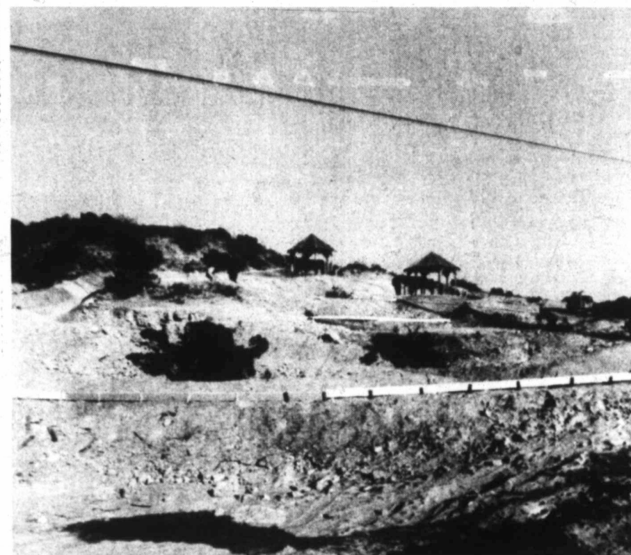
READY TO POUR — Finally carved out of the mountain, the park is ready for concrete to be poured into the forms around the runs. Pleasure Pools of San Angelo did the shotcrete, beginning Apr. 21, when this picture was taken.
