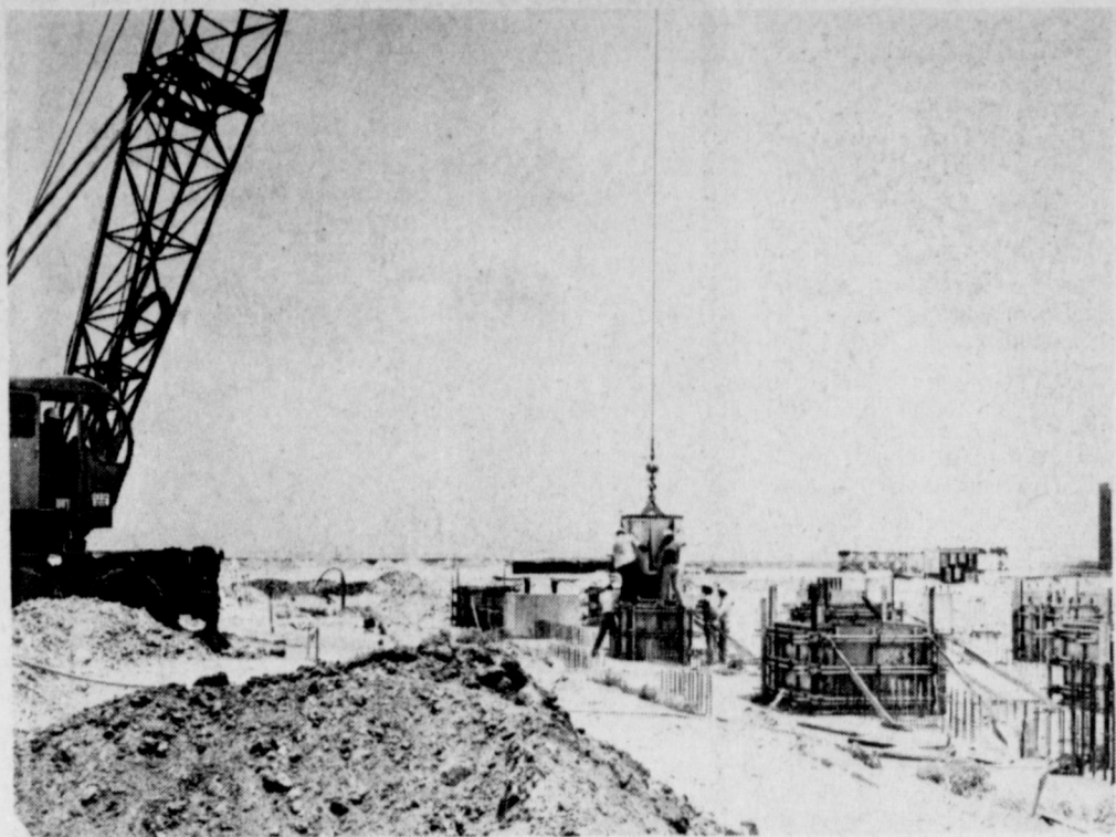
CONCRETE POURED FOR FOUNDATIONS -- At the new Tolk Station, Southwestern Public Service Company's electric generating station, nine miles east of Muleshoe, concrete work is being done at this time. Here the workmen are pouring concrete piers for steel columns. The foundation is for the boiler building and the sub-foundation has just been completed. Concrete will be poured for the turbine building this week.
