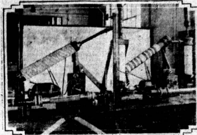
These queer-shaped pipes were used at the U. S. Bureau of Standards automotive laboratory to find the comparative values of various anti-freeze solutions on the market.
