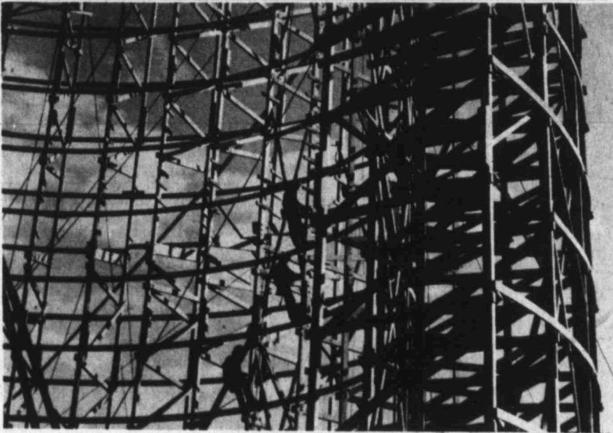
ROLLING HIGH-RISE — Astroworld construction workers create a towering view as they prepare a section of "The Texas Cyclone" roller coaster to be in action this spring. In a major bid for national tourists to Houston, Astroworld is constructing a multi-million dollar Coney Island section to feature the ride, a Texas-sized replica of the 50-year-old New York Coney Island "Cyclone" roller coaster. It is 3,180 feet long, and the ride will reach 60 m.p.h.
