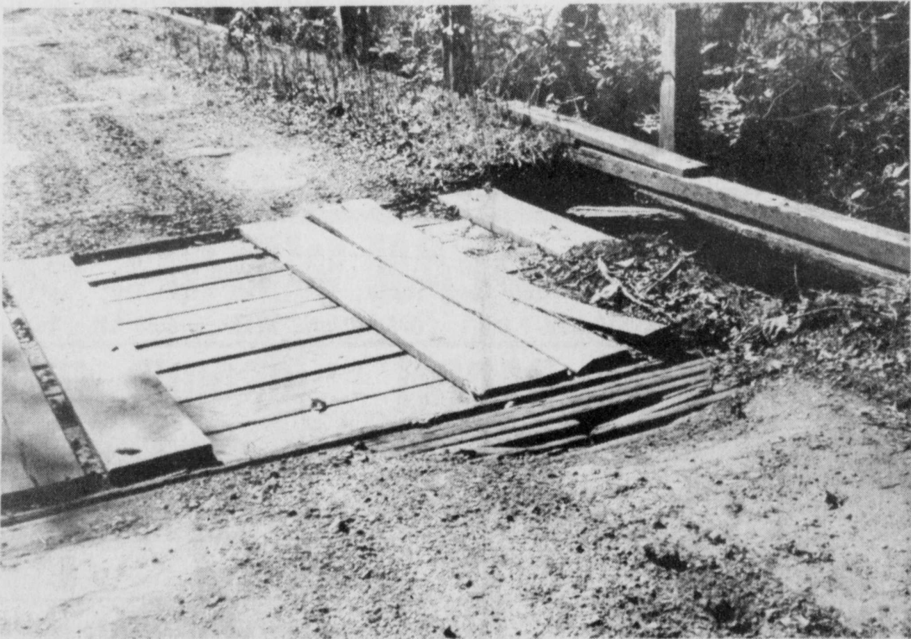
PLANNING STAGES-This bridge located on the old Jolntown highway is in the planning stages for repairs. One of the main support beams has shifted and caused a drop in the surface and several of the timbers have rotted, leaving holes in the bridge. Commissioner Bobby Dickey hopes to have the plans worked out soon. (Staff Photo by Diana Eudy)
