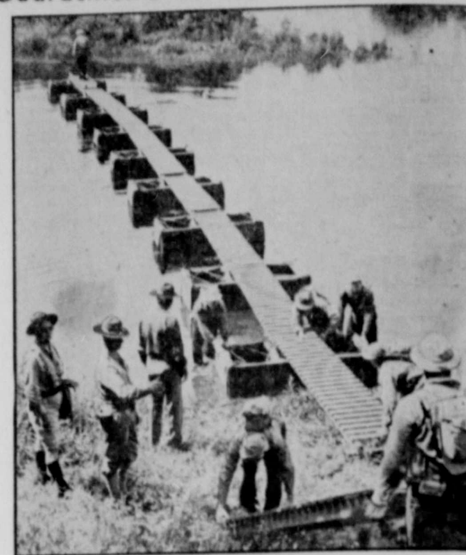
Rhode Island national guardsmen finish work on a floating foot bridge for use by infantry troops during war games in New York.
