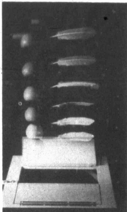
Dropping through a vacuum, a feather and apple fulfill the theory that all objects fall at the same rate of acceleration. But scientists now suggest that a fifth force may counteract gravity, making objects fall at different rates.
