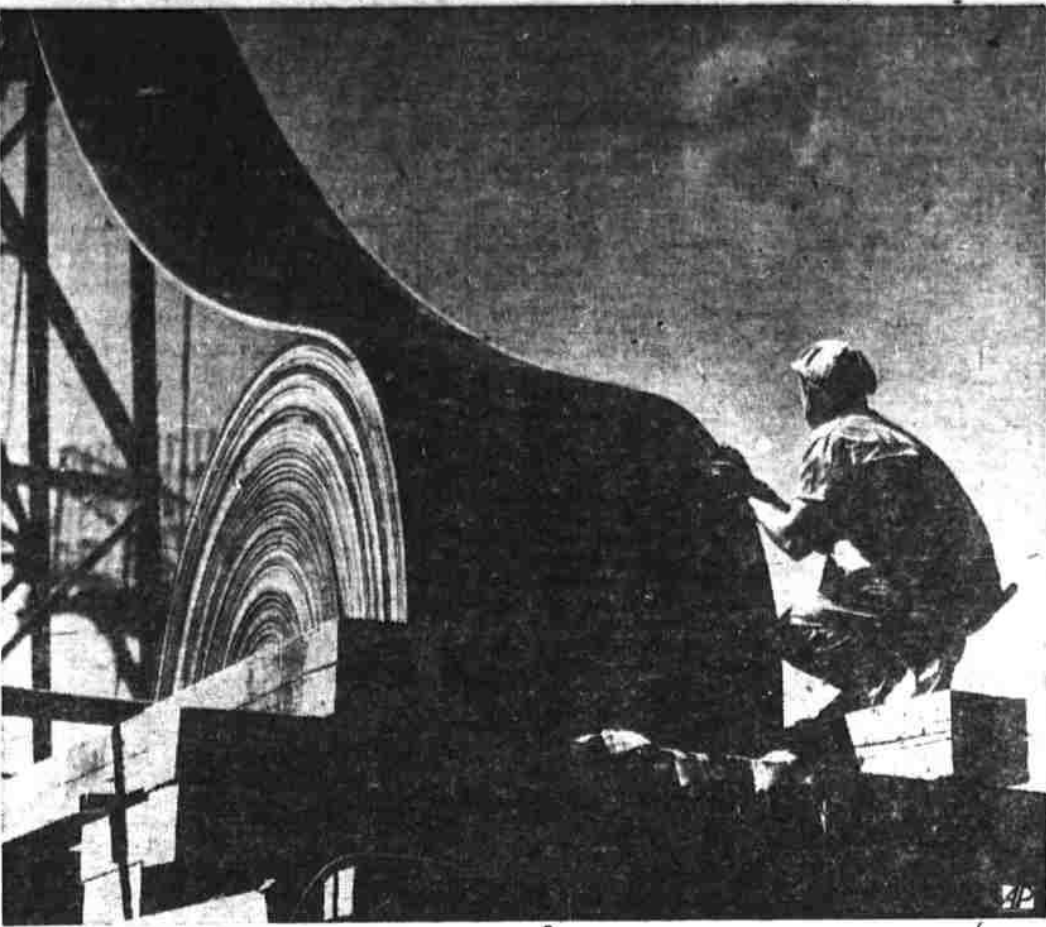
GIANT BELT AT GIANT DAM —Grand Coulee—carries 30,000 tons of sand and gravel daily. Eighty tons of rubber and cotton comprise the belt which is 48 inches wide, two miles long.
