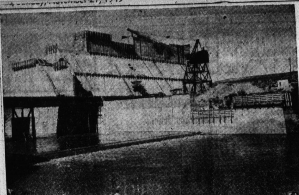
SPILLWAY FOR CENTRAL TEXAS RIVER—This concrete spillway of the Whitney Dam rises above the Brazos River near Waco, Tex. The dam is part of the flood control project on the Central Texas river being built by the Galveston District of the Corps of Engineers. (AP Photo)
