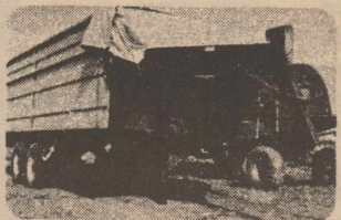
Extra large Rhoman Hopper doors are equipped with a heavy duty rack and pinion operating mechanism.
