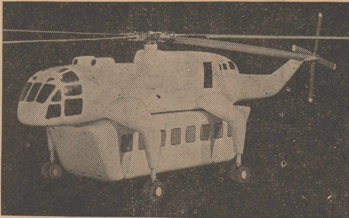
FROGLIKE —Resembling a frog straddling a bus, this is a model of the proposed British Westland helicopter. Designed to provide a three-way lift, the odd whirlybird can be used as an aerial crane, short-haul transport or carrier for utility pods.
