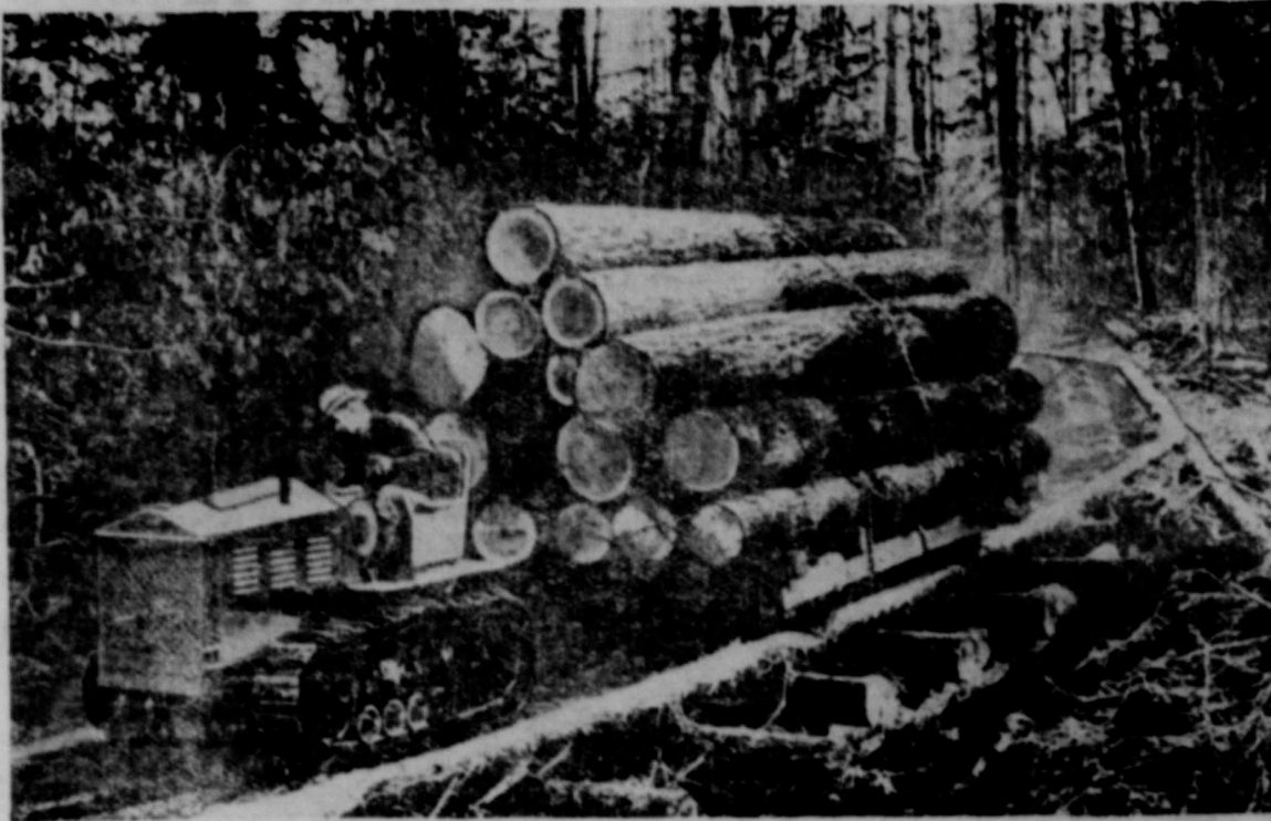
Heavy power machinery and other mechanical equipment has largely revolutionized logging methods in the past decade. An example is the Naylor logging camp near Ravensdale in western Washington. A 110-horsepower caterpillar tractor is able to pull a 10-ton load of logs on a flat car which runs on wooden rails.
