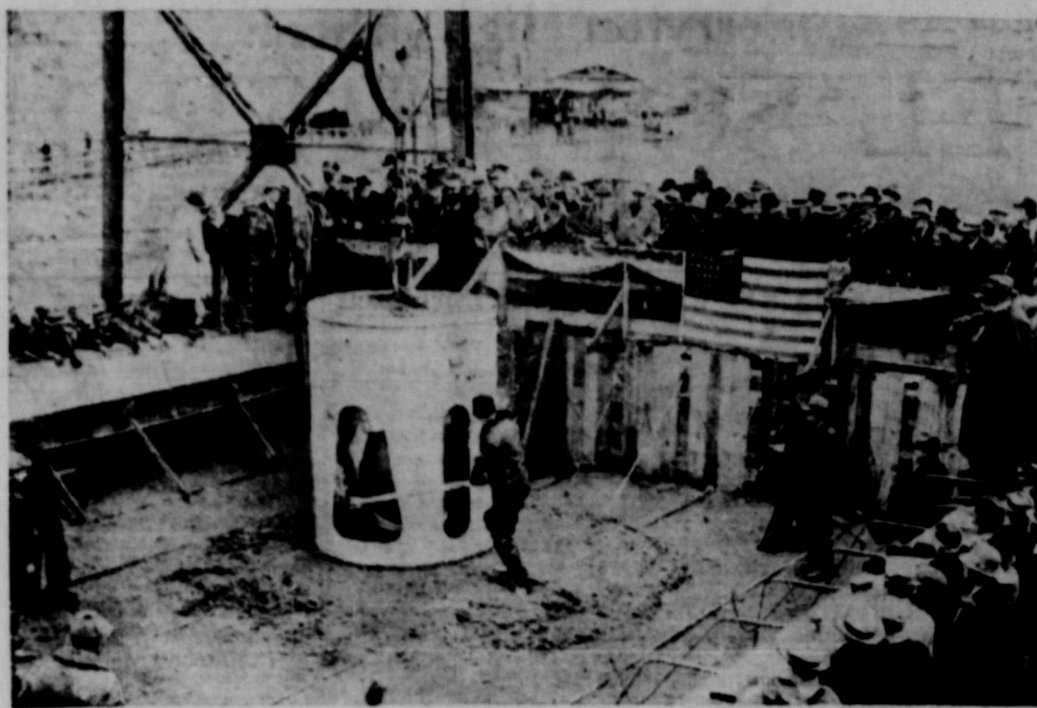
Governor Martin of Washington, in dungarees, throwing the lever for the pouring of the first bucket of concrete in the Grand Coulee dam project. Eleven million square yards of concrete will be needed for the foundation of the $24,000,000 dam.
