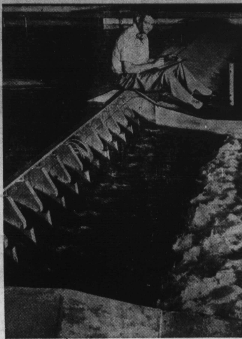
MAN-MADE RIVER—An Army engineer sits on top of a model of Gavin's Point Dam on the Missouri River to make notes on the effectiveness of the design of a spillway and stilling basin now under construction in South Dakota. From such accurately scaled models at the Vicksburg Waterways Experiment Station engineers study and test proposed construction to improve rivers and harbors.
