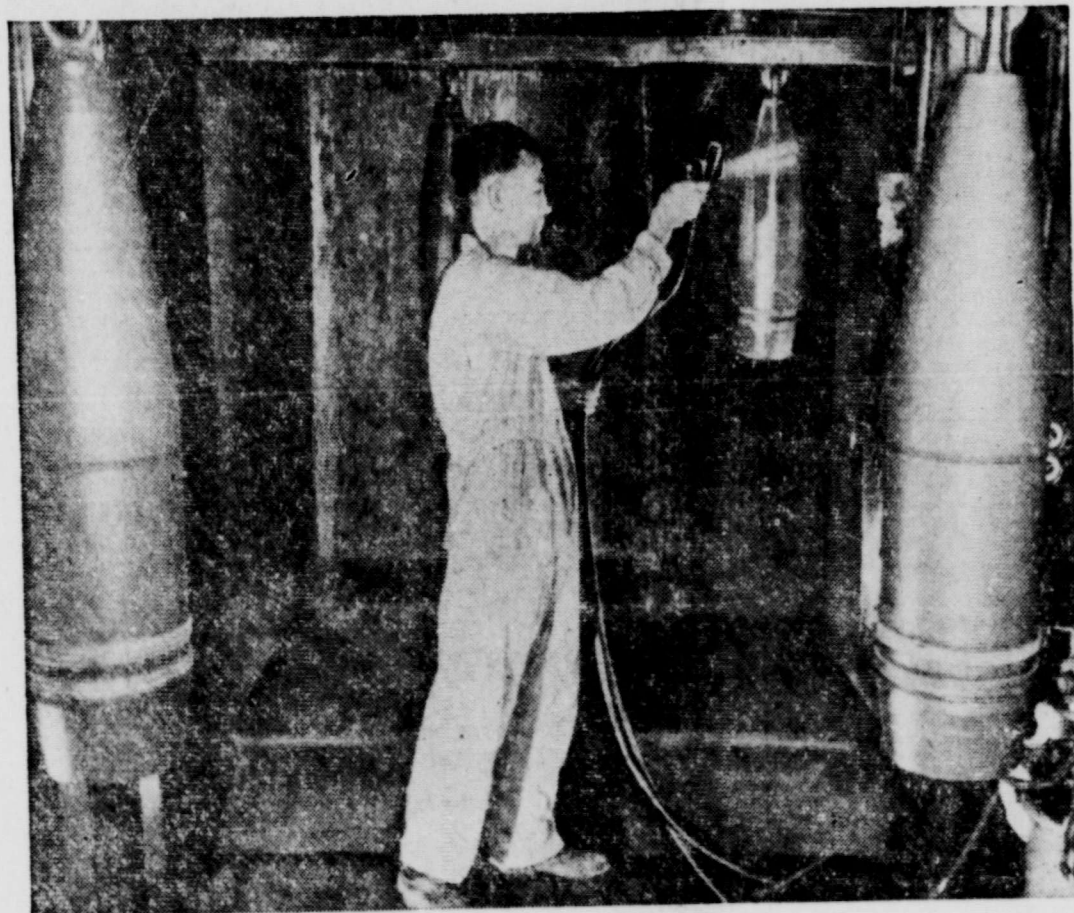
UNCLE SAM'S WORKSHOP—A workman applies a new coat of paint to projectiles after sand-blasting removed the old paint at the giant Red River Arsenal in Texarkana, Tex. After painting, the projectiles are ready to be stenciled and stored in an ammunition igloo, ready for shipment to a battle zone. (Defense Dept. Photo from Acme.)
