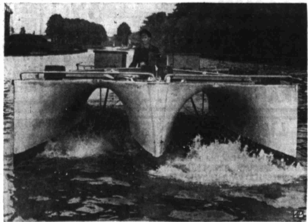
A NAUTICAL NOVELTY — A 20-foot self-powered model of a revolutionary ship's hull is demonstrated on the Thames river at Hampton, England. The trimaran hull is primarily designed to overcome some of the problems of the conventional ship's hull.
