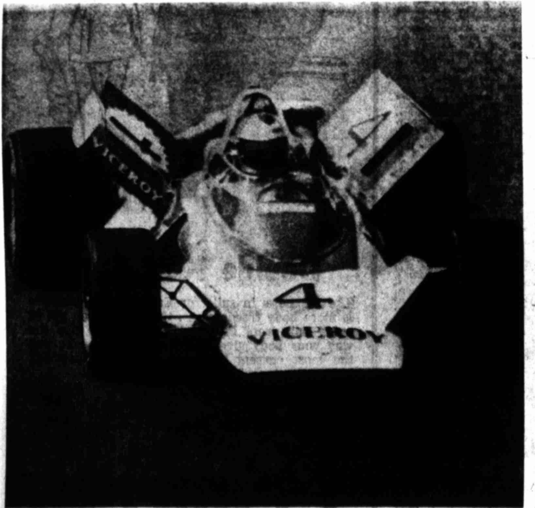
NEW RACING CAR GOES THROUGH TESTS — Mario Andretti drives a stubby winged racing car of revolutionary design in a demonstration run at Ontario, Calif., Motor Speedway. The car, designed by Maurice Philippe of England, was introduced by Parnelli Jones and Vel Miletich, who are building six of the cars for the Indianapolis 500. The car has two wings mounted
