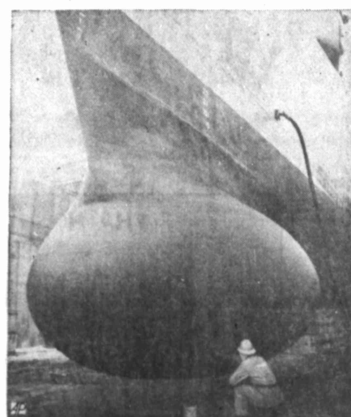
BUBBLE NOSE —Bow dome of inch-thick rubber, 10 feet high, 20 feet wide and 37 feet long, contains sonar gear of destroyer Willis A. Lee at Boston shipyard.
