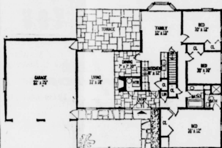
Floor plan of the "House of Wood" shows the convenient location of rooms which open onto the terrace. All bedrooms are off by themselves for privacy.
