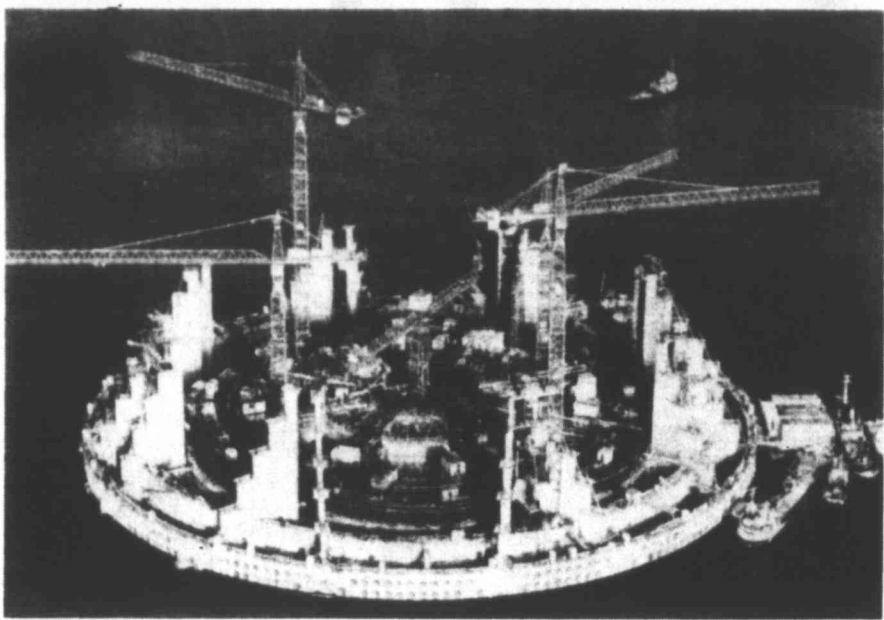
GIANT OIL PLATFORM — The huge Ninian Central platform being built for Chevron Oil's Ninian North Sea oil field is moored in Loch Carron, Scotland, recently with its massive base structure showing above the water. When completed it will weigh over 400,000 tons. The indents on the side walls help resist sea pressure.
