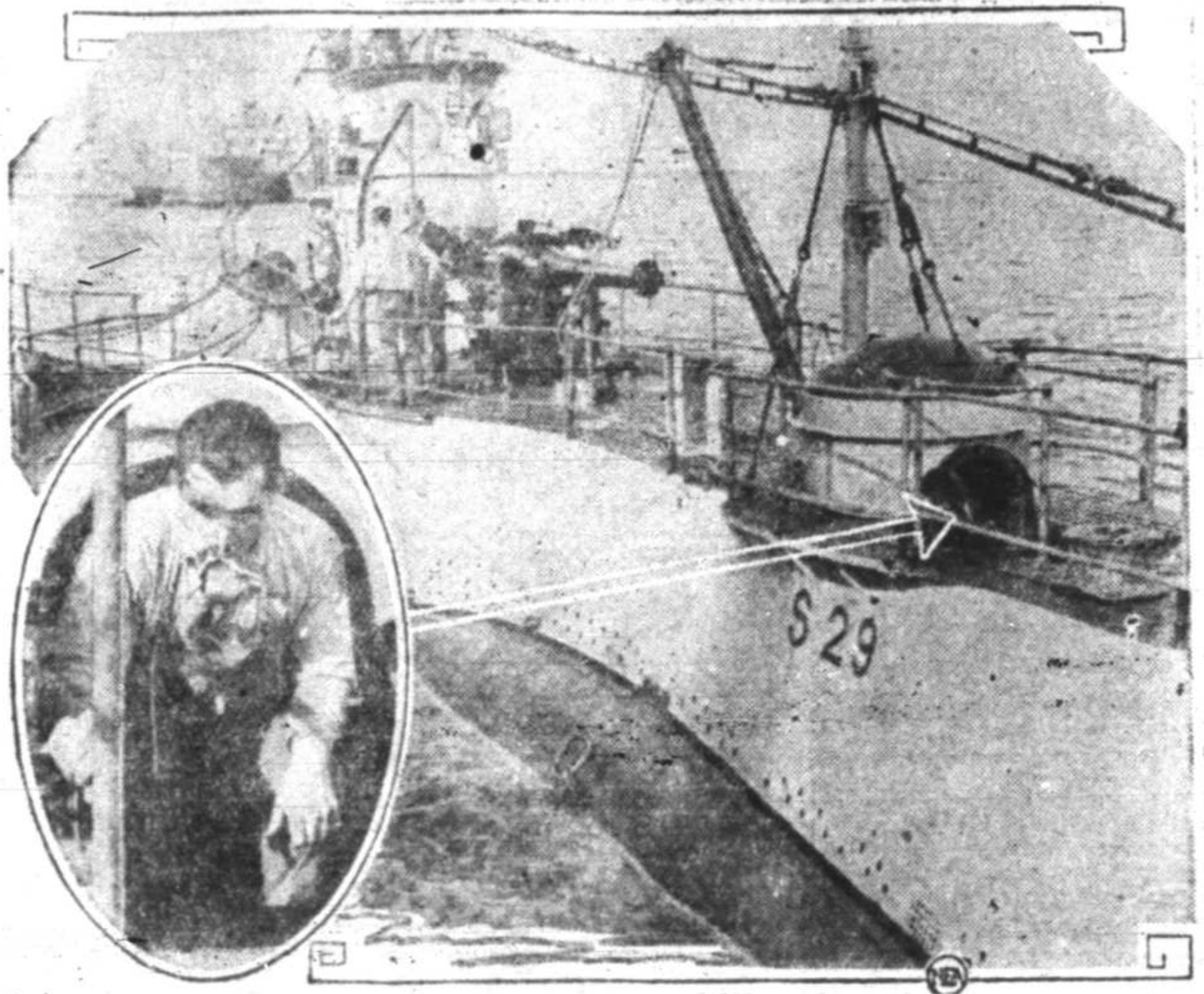
Here is the U. S. navy's S-29 which has become a test ship for submarine safety devices at the San Diego naval base. At the left, Mechanist Mate H. L. Kirby is demonstrating how a sailor, wearing a "mechanical lung," escapes from a sudden sub via the turret-like escape lock, indicated by the arrow. One of the steel rings for the quick lifting of sunken subs, eliminating the necessity for weary tending through the mud by divers in order to pass chains underneath, may be seen on the S-29's hull.
