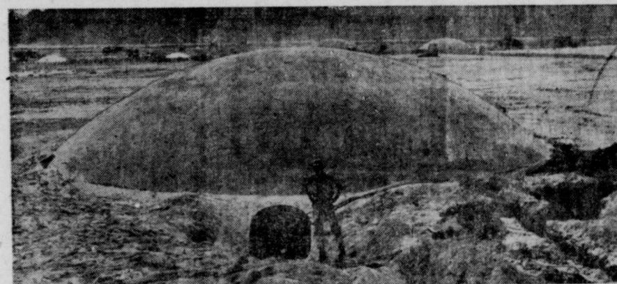
DOMES SHELTERS, a new design whose low cost and easy construction would adapt it to mass production, were tested at the Operation Plumbbob atomic tests in Nevada at pressures from 20 to 70 pounds per square inch. The lower photo shows one of the domes which was deliberately tested at a pressure so great that it would fall, so its weaker points could be studied. (NTO Lookout Mountain Lab Photo)
