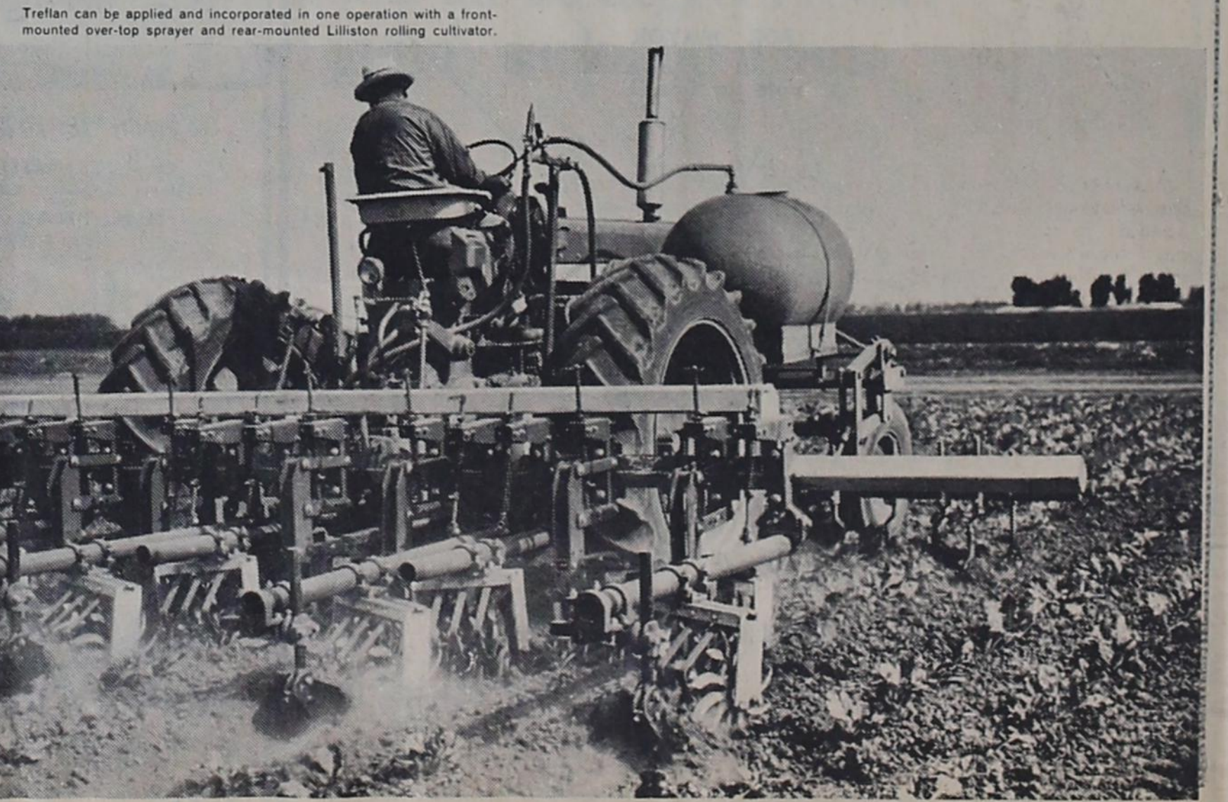
Treflan can be applied and incorporated in one operation with a front-mounted over-top sprayer and rear-mounted Lilliston rolling cultivator.
