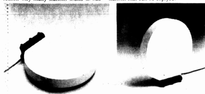
THE BEST-PERFORMING COMPACT FM ANTENNA on the market today may be Terk Technologies' "Pi" FM antenna (pronounced "PIE"). This unusual, disc-shaped antenna is about the size of a compact disc and rests in the horizontal position for omni-directional reception or vertically to tune in weaker-powered FM stations.
