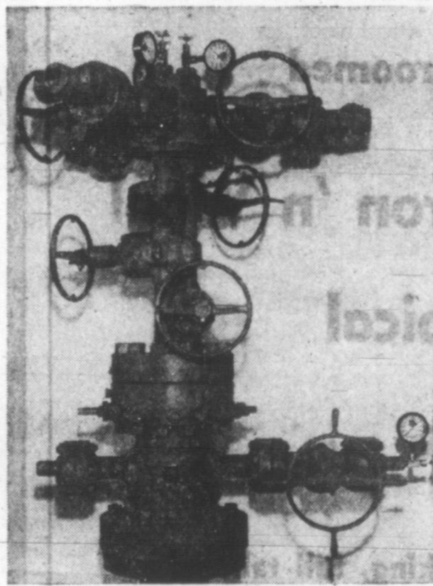
TRIPLE CONNECTION COMPLETION TREE using Cameron gate valves
