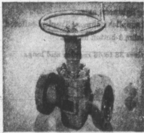
THE TYPE "F" W.O.G.M. VALVE The new Cameron Type "F" API Gate Valve—brand new sealing principle (the valve with the rotating seat) produces the longest wear without repair. Pressure ratings through 15,000 p.s.i. W.P.
