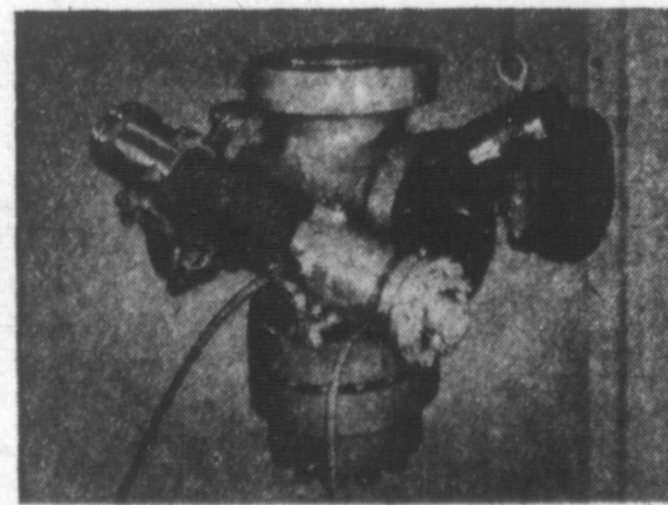
THE BALANCED DESIGN BLOWOUT PREVENTER Preview of the Type "F" Cameron Blowout Preventer — greatest strength, highest working pressures (to 15,000 p.s.i.) ever developed. Requires less pressure to operate, new convenience in ram changing.
