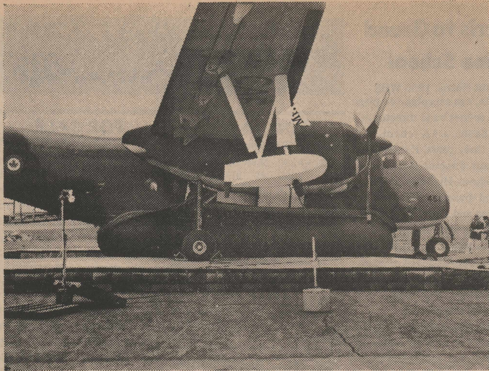
SOFT LANDING is assured for this Canadian Department of National Defence CC-115 Buffalo aircraft which is testing the Air Cushion Landing System, a program sponsored jointly by the United States and Canadian governments at Textron's Bell Aerospace Division, Buffalo, N.Y.
