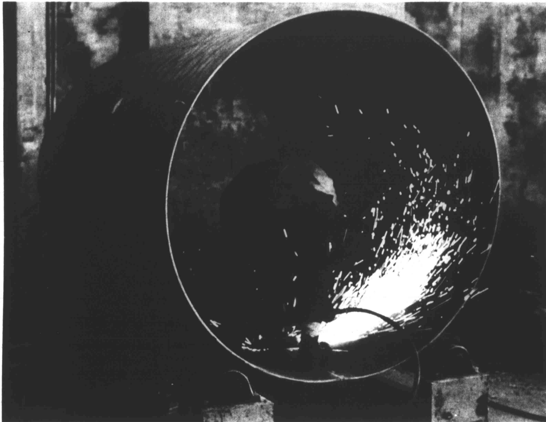
MAKING A TUBE — A flat piece of steel must be rolled and welded to make a tube for tank trailers. The welds are first made by hand to hold the tube
