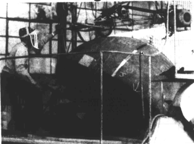
JOIN IT — The Steel is first welded by hand, then by machine to make sure no joint has an imperfection. Above, a machine rotates the head of a tank so a worker can grind and weld on it.
