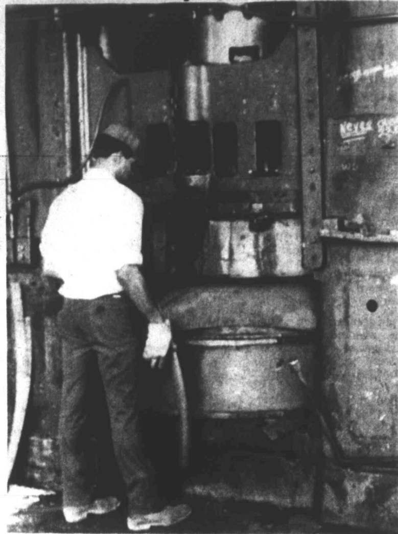
MAKING CURVES — An employee operates a giant press which shapes the steel into curved surface so the cones or heads of the tanks can be made. Other machines roll the steel into tubes.
