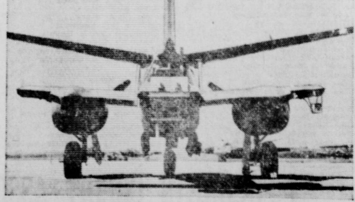
WINGLESS WONDER—Shorn of wings, this B-26 bomber has been ground-taxed for vital skid tests at the Wright-Patterson Air Force Base, in Dayton, O. At top, the plane is raced down a runway in a simulated landing which will yield valuable data needed to design lighter, stronger and smaller landing gears. The bottom view shows where the B-26's wings have been clipped to avoid lift. (Dept. of Defense Photo from Acme.)
