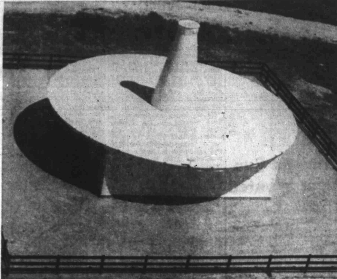
Located 10 miles north of Webb AFB near Fairview off the Gail Road, this foreign appearing object is a radio guidance range for aircraft. Nestled among the cotton fields, it could easily be mistaken for a flying saucer or rocket ship from Mars. The Federal Aviation Agency calls the aid to air navigation a "very high frequency omnidirectional radio range."
