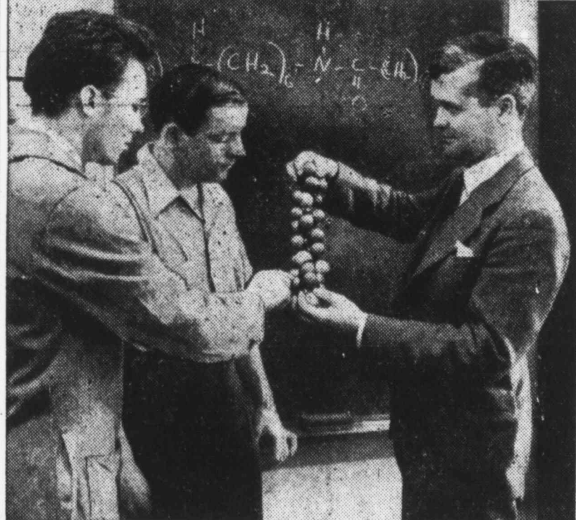
Chemistry Professor Malcolm Dole (right) explains to students what a molecule of nylon looks like. The chemistry department works in co-operation with the engineering department.
