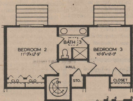
UPPER FLOOR BEDROOMS TYPICAL UNIT B-2 APPROX 465 sq ft
