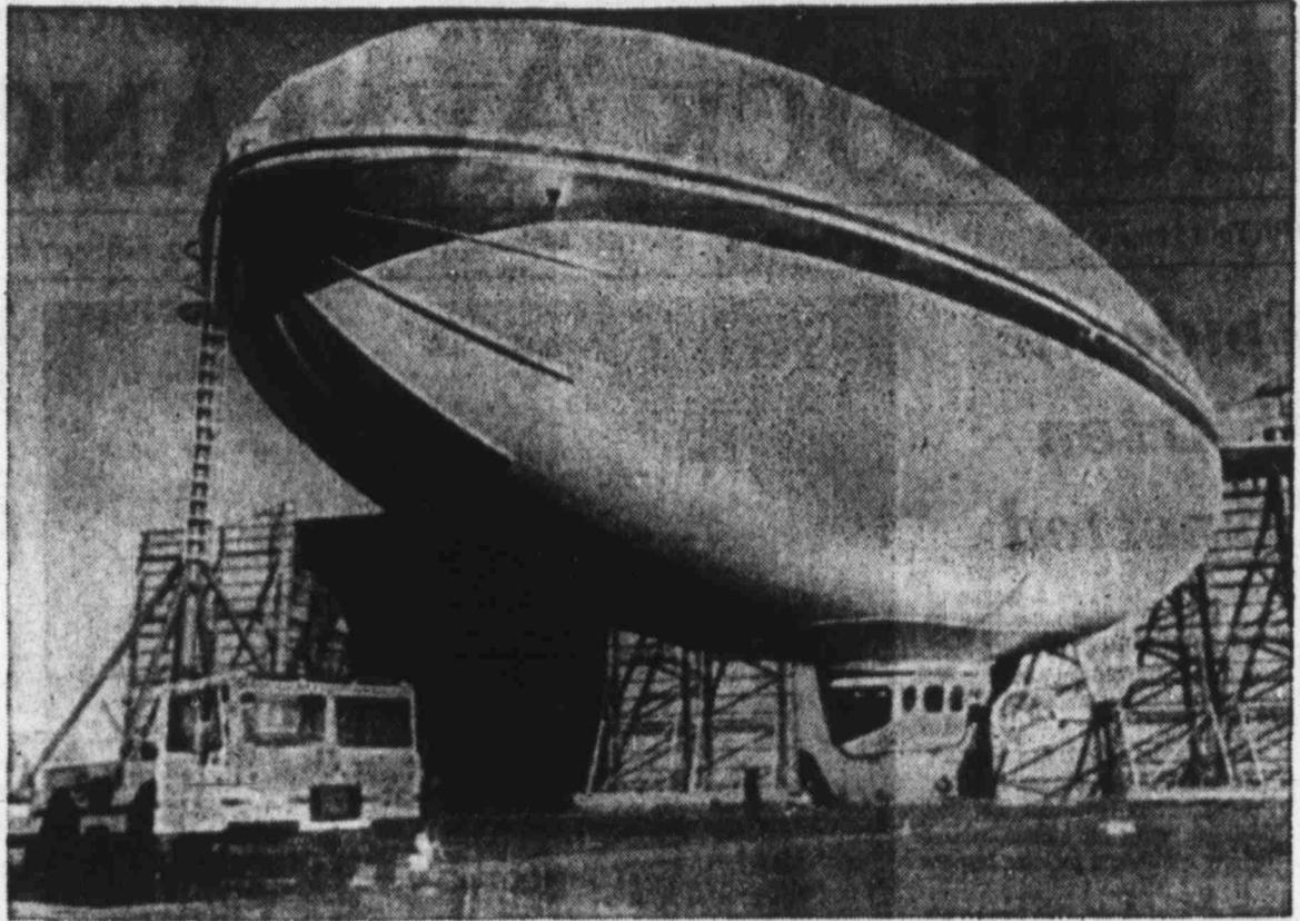
NEW COMMERCIAL AIRSHIP — The AD500, the first commercial airship to be built in Britain for nearly 50 years, takes off for a recent test flight from Cardington, Bedfordshire. It has been designed by Aerospace Developments, and costs around 600,000 English pounds. The AD500 is capable of lifting 2½ tons or carrying 10 passengers. (AP Laserphoto)
